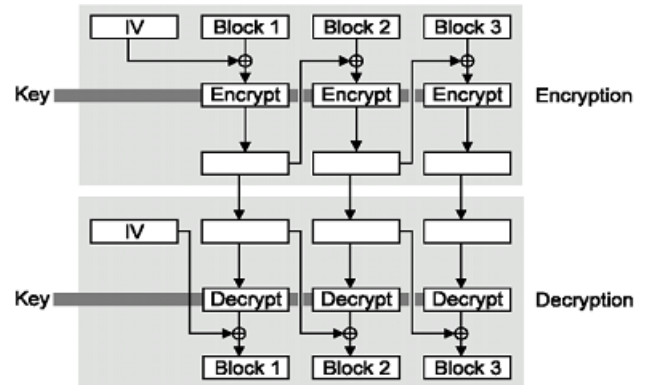
Mode CBC
